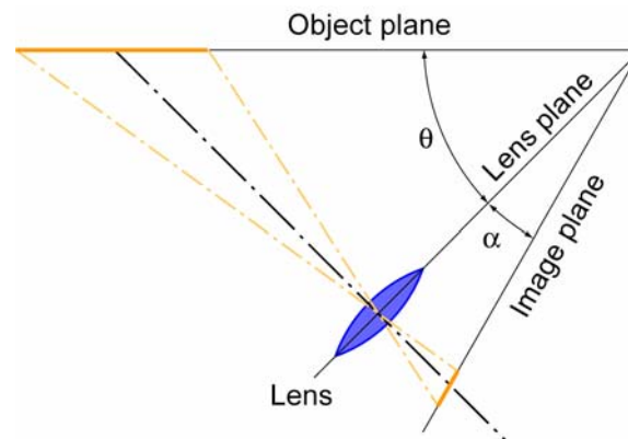
Figure 6: Scheimpflug Condition.
